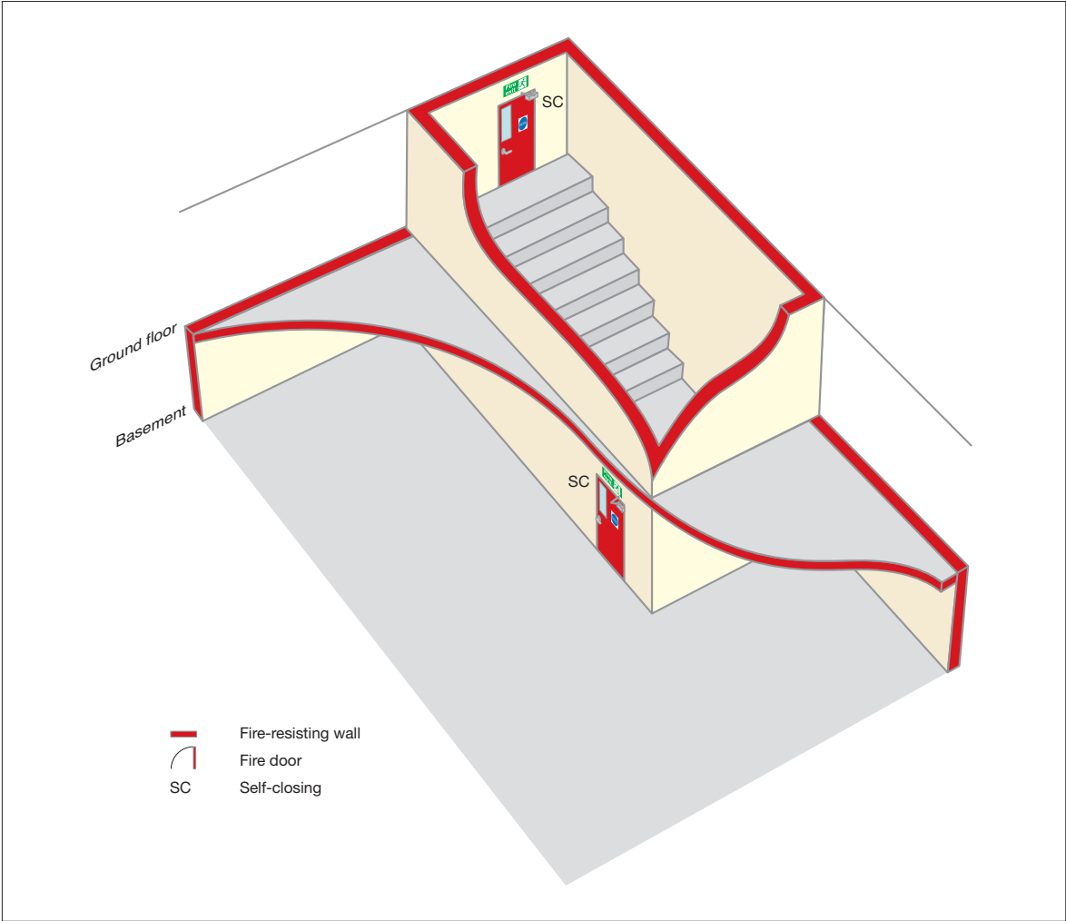
Figure 33: Basement protection
