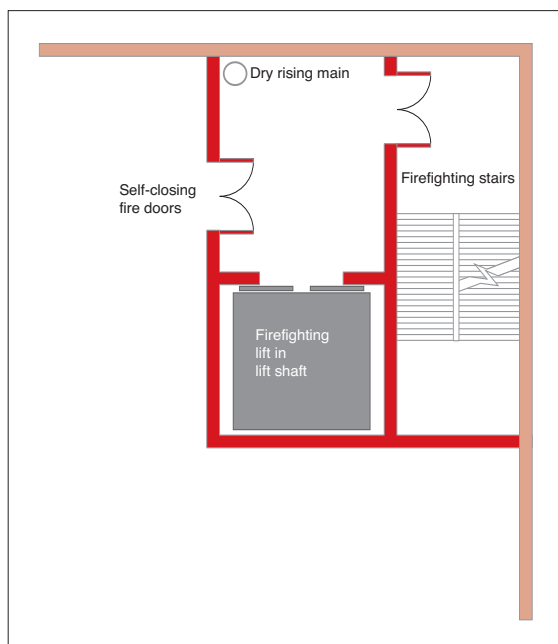
Figure 20: Firefighting shaft
