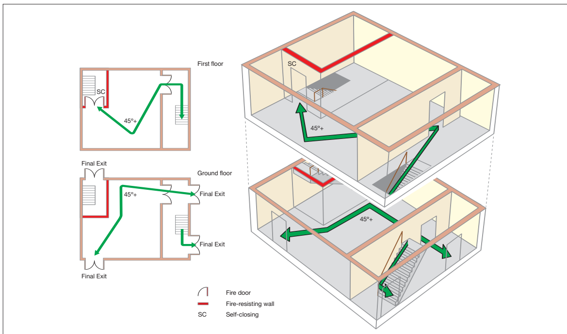
Figure 45: Two-storey premises: lower risk premises (e.g. church hall)
